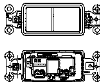
3-WAY WITH IL. LAMP
