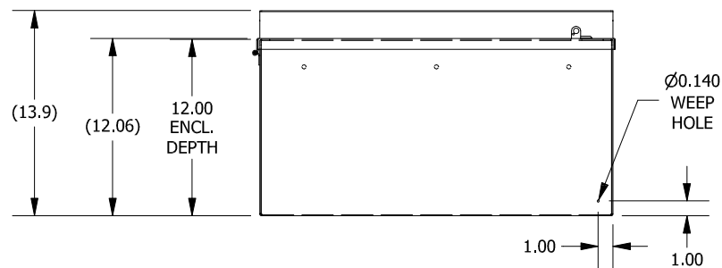
BOTTOM VIEW
