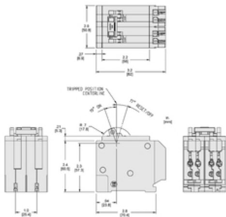
HOMT Quad Tandem Circuit Breaker Two spaces required. All dimensions are approximate. Also see technical documentation.
