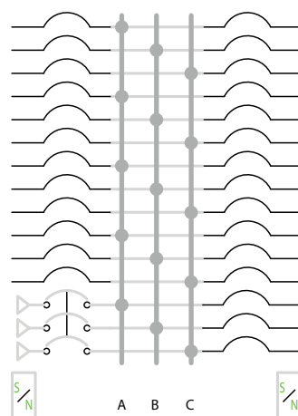
125 A Max. Branch Mounted Main Circuit Breaker
