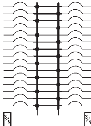
400 A or 600 A PowerPacT L-Frame Main Circuit Breaker with Sub-feed Circuit Breaker
