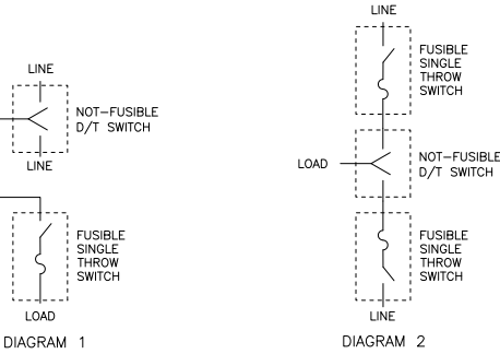
DIAGRAM 1 AND 2 ILLUSTRATE METHODS OF APPLYING FUSES TO DOUBLE THROW SWITCHES WHEN REQUIRED.
