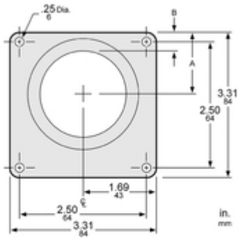
A Hub Mounting Dimensions
