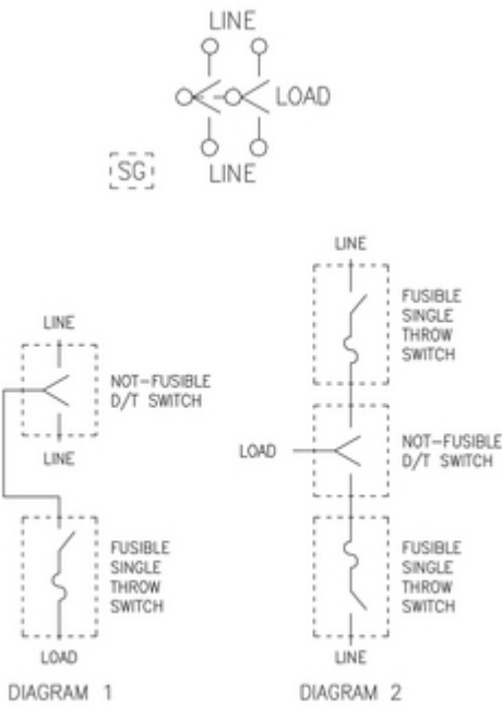
DIAGRAM 1 AND 2 ILLUSTRATE METHODS OF APPLYING FUSES TO DOUBLE THROW SWITCHES WHEN REQUIRED.
