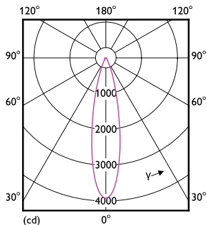
Light Distribution Diagram - 8.5PAR30S/COR/927/F25/D/P/ULW/T20 6/1FB
