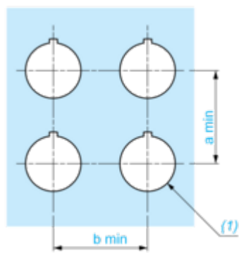
(1) Diameter on finished panel or support
