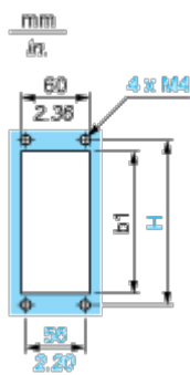
Panel cut-out
