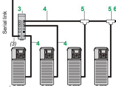
Example of serial link architecture
