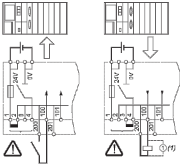
(1) Inductive load
