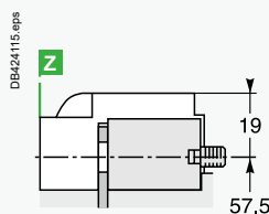
Distribution connector, 6 cables
