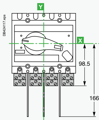
Distribution connector, 6 cables
