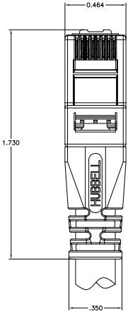
PLUG & BOOT DETAIL
