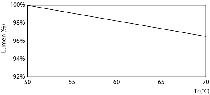
Lumen Maintenance Diagram - 8.4T8/MAS/48-840/MF16/G/DIM UE 25/1
