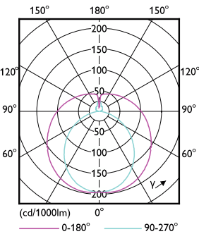
Light Distribution Diagram - 8.4T8/MAS/48-840/MF16/G/DIM UE 25/1
