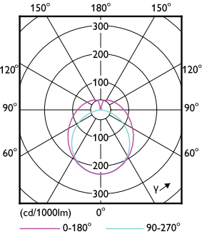
Light Distribution Diagram - 11.5T8/MAS/48-835/MF21/G/DIM UE 25/1
