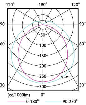
Light Distribution Diagram - 10PL-L/COR/24-5CCT/MF11/G/4P 10/1
