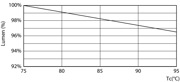
Lumen Maintenance Diagram - 10PL-L/COR/24-5CCT/MF11/G/4P 10/1
