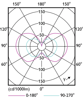
Light Distribution Diagram - 18-12-9CC/LED/3PW/3CCT/E26 BB 6/1
