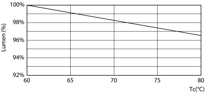
Lumen Maintenance Diagram - 22CIR/CNG/16-4CCT/IF26/P/G10q 6/1
