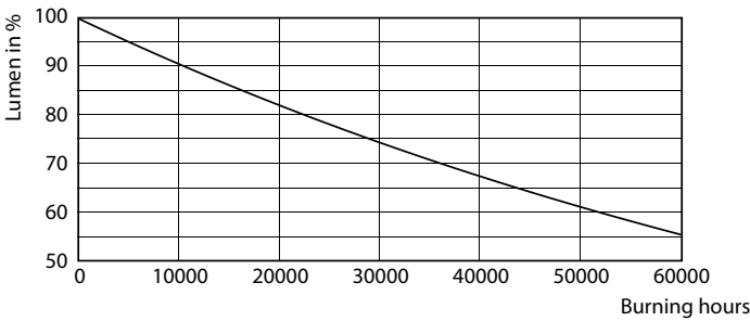
Lumen Maintenance Diagram - 22CIR/CNG/16-4CCT/IF26/P/G10q 6/1
