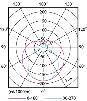
Light Distribution Diagram - 10.5T8/COR/48-835/IF15/G/DIM/BAA 25/1
