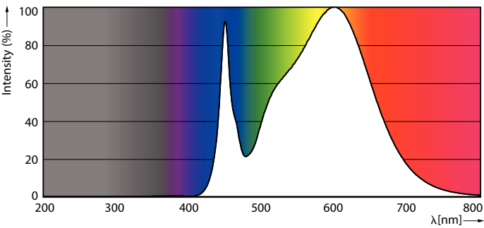
Spectral Power Distribution Colour - 10.5T8/COR/48-835/IF15/G/DIM/BAA 25/1
