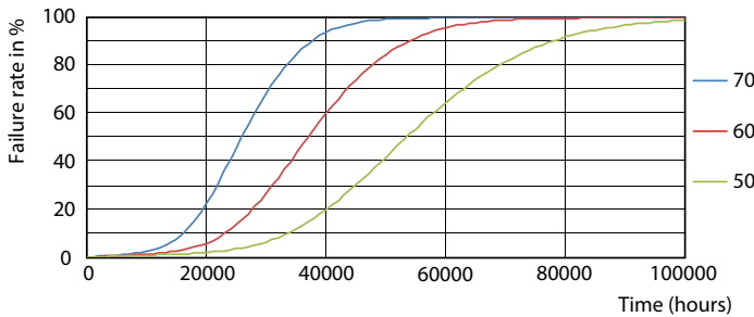
Life Expectancy Diagram - 10.5T8/COR/48-835/IF15/G/DIM/BAA 25/1
