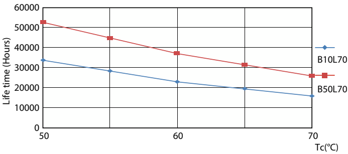
Life Expectancy Diagram - 10.5T8/COR/48-835/IF15/G/DIM/BAA 25/1
