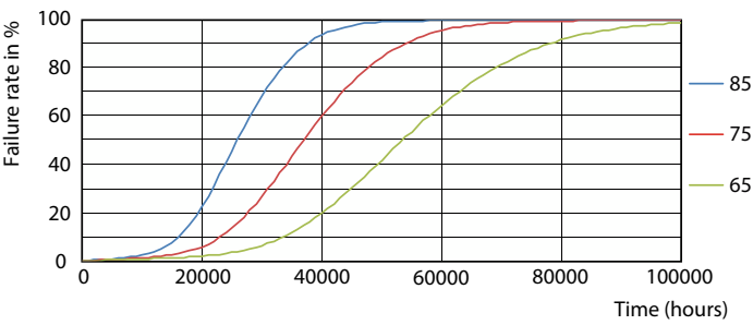
Life Expectancy Diagram - 17PL-L/COR/22-830/MF22/G/4P 10/1
