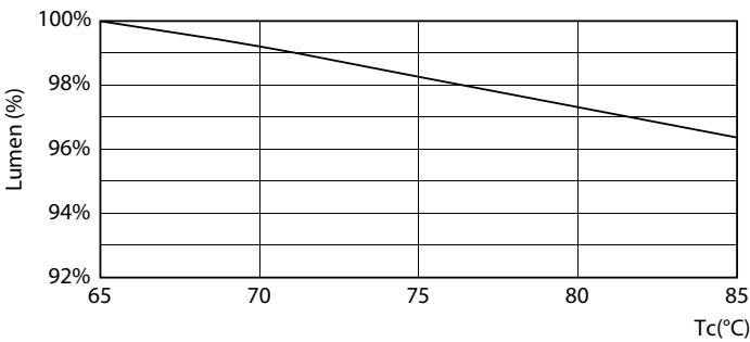
Lumen Maintenance Diagram - 17PL-L/COR/22-830/MF22/G/4P 10/1
