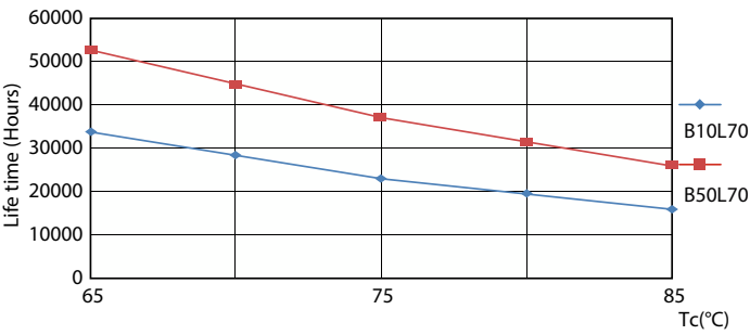
Life Expectancy Diagram - 17PL-L/COR/22-830/MF22/G/4P 10/1
