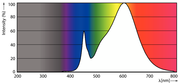
Spectral Power Distribution Colour - 17PL-L/COR/22-830/MF22/G/4P 10/1
