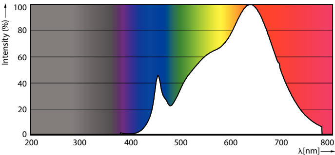
Spectral Power Distribution Colour - 6.3MR16/LED/F25/930/D/EC/12V T20 10/1FB
