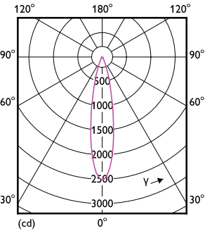
Light Distribution Diagram - 6.3MR16/LED/F25/930/D/EC/12V T20 10/1FB
