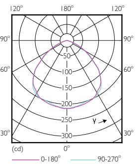
Light Distribution Diagram - 13.5PAR38/PER/GREEN/G/E26/ND/ULW 3/1PF
