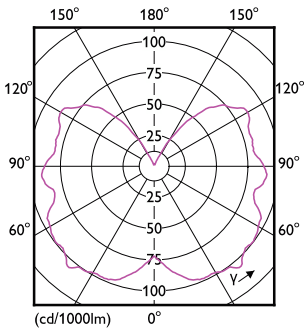
Light Distribution Diagram - 3.5A15/VIN/820/E26/Amber/G/SP D 4/1PFT20
