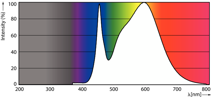
Spectral Power Distribution Colour - 145HB/LED/840/D WB UDL BB G2 4/1
