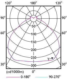
Light Distribution Diagram - 145HB/LED/840/D WB UDL BB G2 4/1
