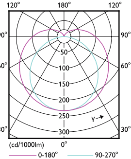
Light Distribution Diagram - 14.5T8/48-835/MF20/MC IA 10/1
