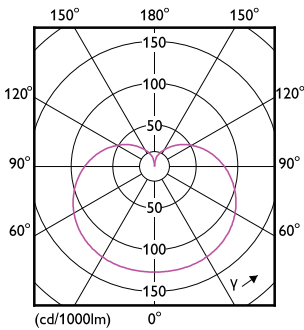
Light Distribution Diagram - 16A19/PER/927-22/P/E26/WG 6/1FB T20
