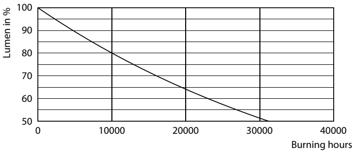
Lumen Maintenance Diagram - 16A19/PER/927-22/P/E26/WG 6/1FB T20
