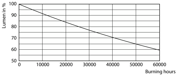
Lumen Maintenance Diagram - 12AR111/LED/927/S8/DIM/EC 12V 6/1FB
