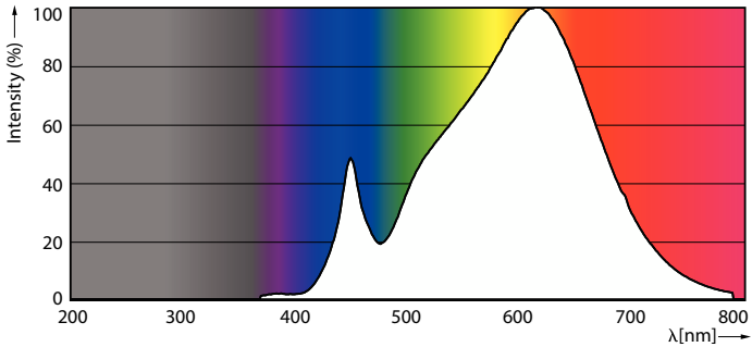
Spectral Power Distribution Colour - 20AR111/LED/930/F25 DIM 12V 6/1FB
