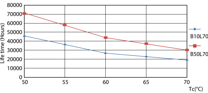
Life Expectancy Diagram - 13T8-6U/MAS/24-850/IF21/P/DIM 10/1
