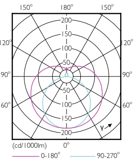
Light Distribution Diagram - 11T5HE/34-835/IF14/G/DIM 10/1
