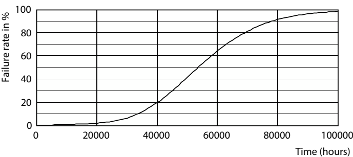
Life Expectancy Diagram - 8T5HE/22-850/IF10/G/DIM 10/1
