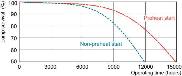
Life Expectancy Diagram - PL-T 57W/841/A/4P 1CT/5X10BOX ALTO
