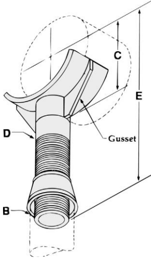
Fig. 875 ADJUSTABLE PIPE SADDLE SUPPORT
