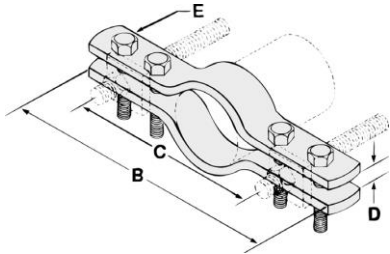
Fig. 590 FOUR BOLT UNDERGROUND PIPE CLAMP
