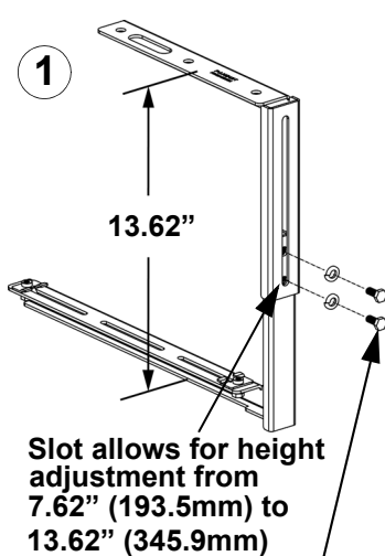
TYPICAL INSTALLATION WITH THREADED ROD
