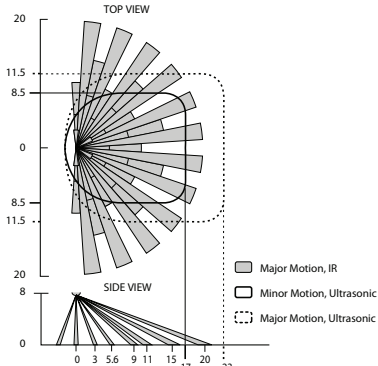
Extended Range Lens for Multi-Tech Models with 180° Mask (Black)
