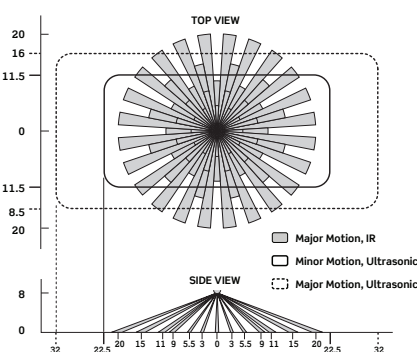
Extended Range Lens for Multi-Tech Models (Black)
