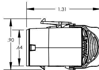
LEVITON ATLAS-X1 CAT 8 SHIELDED JACK
