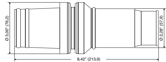
Male Connector Housing
