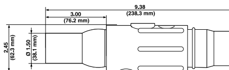
Ball Nose In-line Latching Female Connectors - Crimped
