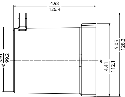
Panel Receptacle Housing
