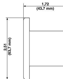
Female Protective Cap
