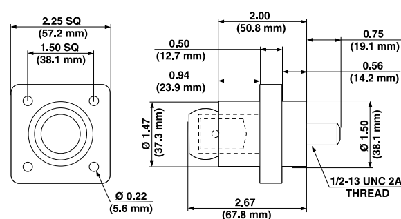
Female Double Set Screw Panel Receptacle
