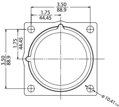
Panel Receptacle Flange
