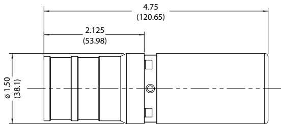
Female Contact
