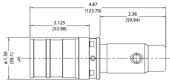
Male Contact
