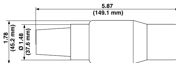
Female Vulcanized Plug - Crimped
