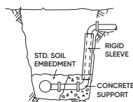
Rigid sleeve for any trench (concrete must support sleeve)
