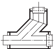
Combination Wye & 1/8 Bend Soc x Sp x Soc
