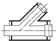
Reducing Wye Soc x Sp x Soc
