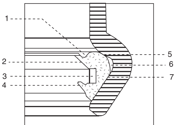
Joint Cutaway
