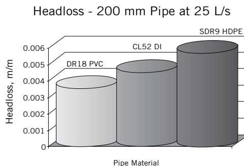
Figure 2 – Pipe Material
