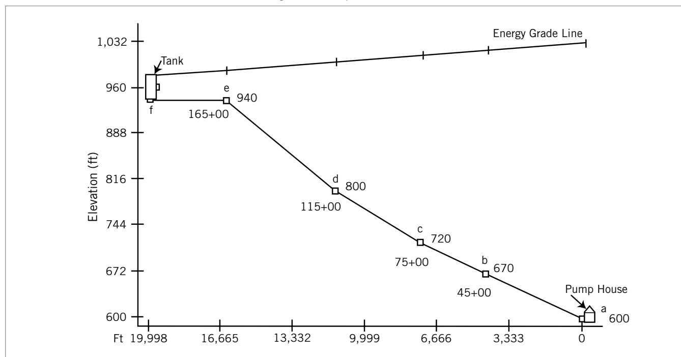
Figure 4 – Pipeline Profile
