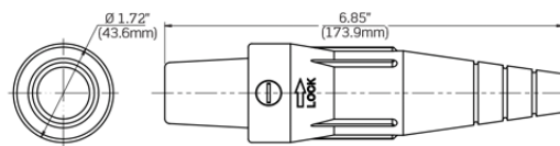
Female Detachable Plug
