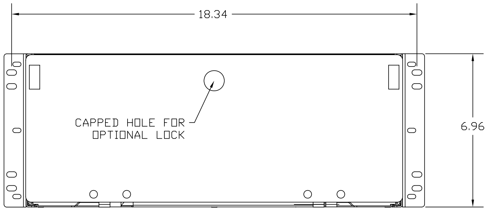
FRONT VIEW
