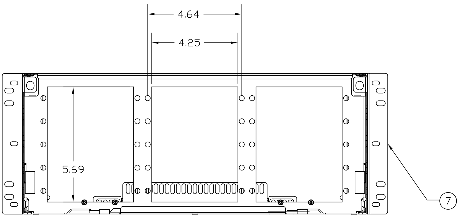
FRONT VIEW (FRONT DOOR NOT SHOWN)
