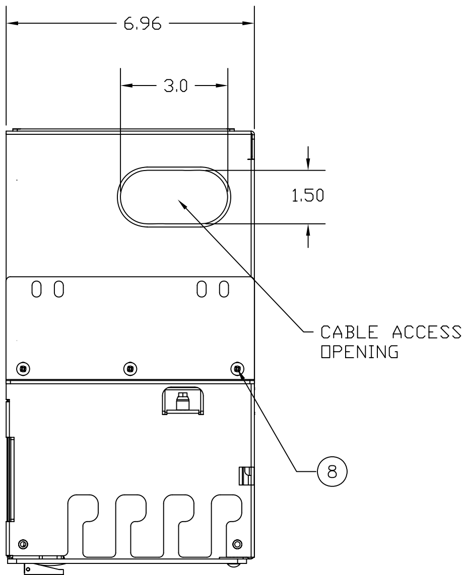
SIDE VIEW
