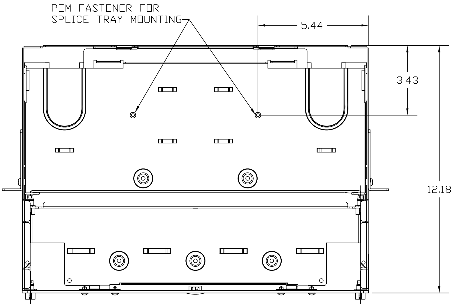
TOP VIEW (TOP REMOVED)
