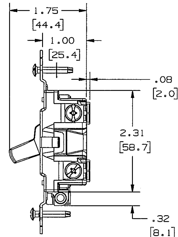
DOUBLE POLE/BACK WIRE & SIDE WIRE
