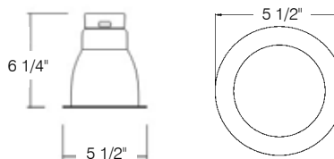
ATV401/W Clear Specular Reflector with White Baffle Code: 79527
