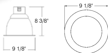
ATV814/W White Wall Wash Code: 79531
