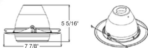
RT604BL/WH/SC Black Baffle with White Eyeball Uses BR/ PAR30 Lamps Order Code: RT604BL/WH/SC
