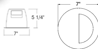
ATV614/W White Wall Wash Code: 79529
