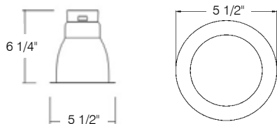
ATV400/C Clear Specular Reflector Code: 79526
