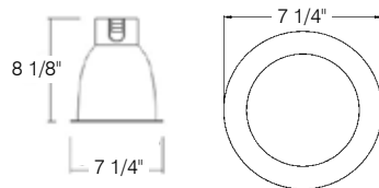
ATV601/W Clear Specular Reflector with White Baffle Code: 79518
