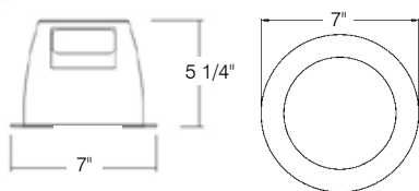
ATH600/C Clear Specular Reflector with White Ring Code: 79501
