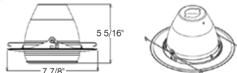
RT603WH/WH/SC White Baffle with White Eyeball Uses BR/ PAR30 Lamps Order Code: 78129
