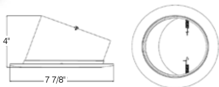
RT600CL/WH/SC Clear Reflector with White Ring Uses BR40, PAR38 Lamps Order Code: 70026
