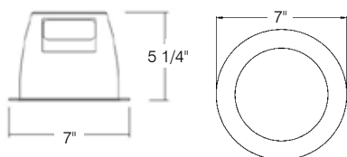
ATH601/W White Baffle with Reflector Code: 79511
