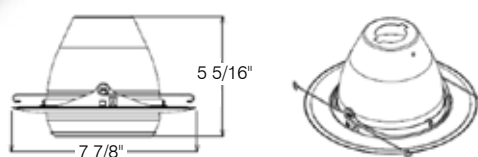
RT604WH/SC White Baffle with White Eyeball Uses BR/ PAR30 Lamps Order Code: 78129
