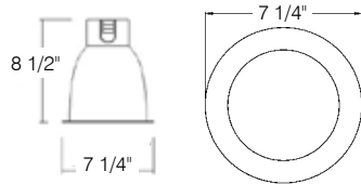
ATV600/C Clear Specular Reflector with White Ring Code: 79517
