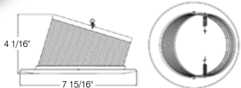
RT602WH/SC White Baffle with White Ring Uses BR40, PAR38 Lamps Order Code: 78154
