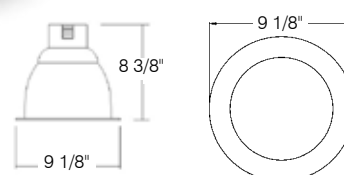
ATV860/W White Flush Lens Code: 79521
