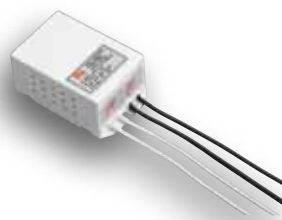
RFA-LV-XFMR-50-EL 120V to 12VAC/50W Electronic Replacement Transformer (Not for use with recessed cans) Order Code: 78225
