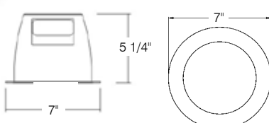
ATH621/C White Baffle with Albalite Lens Code: 79513
