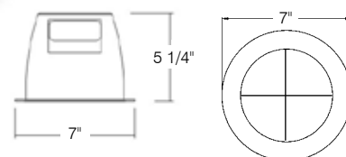
ATH604/C Clear Specular Louver Code: 79512
