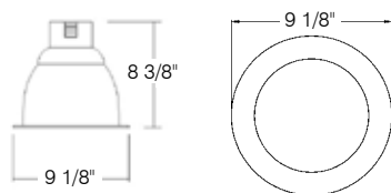
ATV800/C Clear Specular Reflector with White Ring Code: 79520
