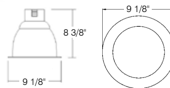
ATV814/C Clear Specular Wall Wash Code: 79530
