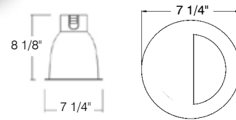
ATV614/C Clear Specular Wall Wash Code: 79528
