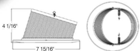
RT602BL/WH/SC Black Baffle with White Ring Uses BR40, PAR38 Lamps Order Code: 70025
