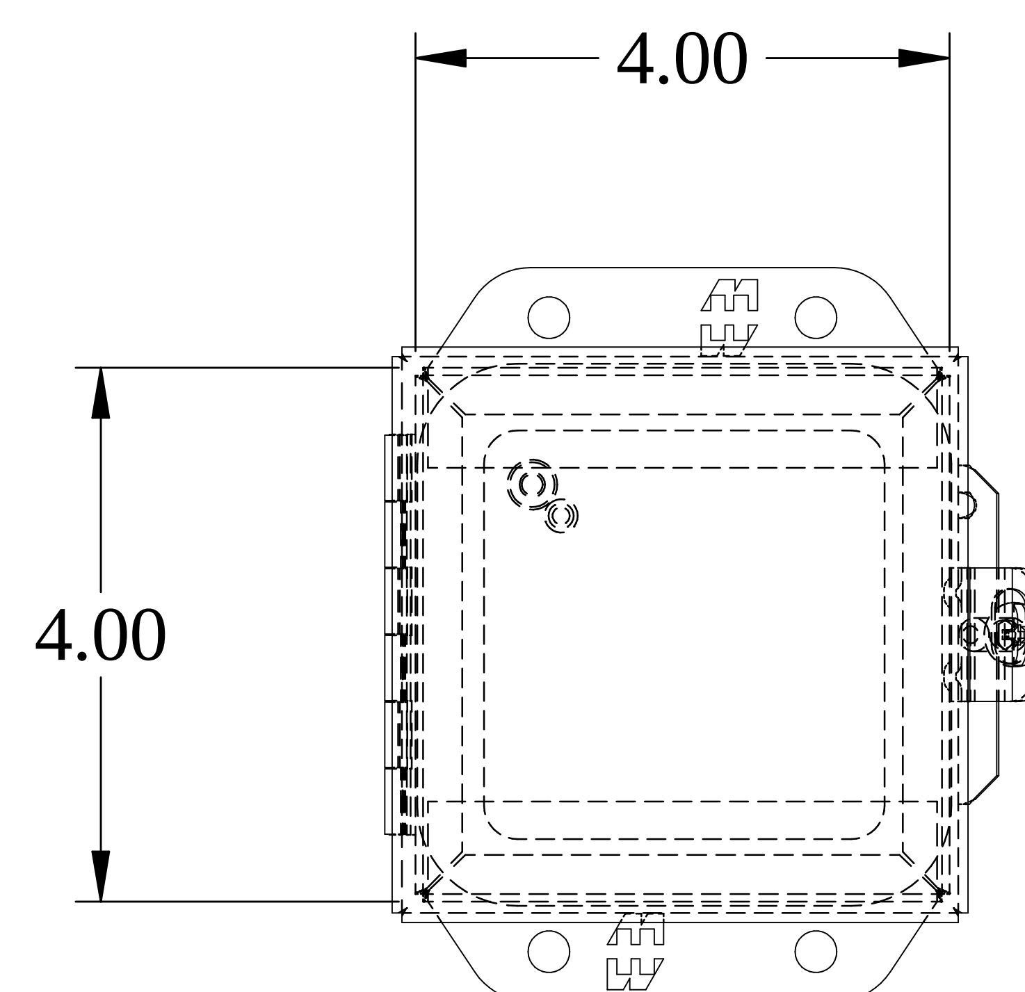
FRONT VIEW
