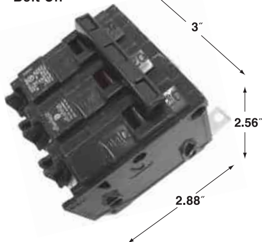
Type BL Three Pole-Bolt On
