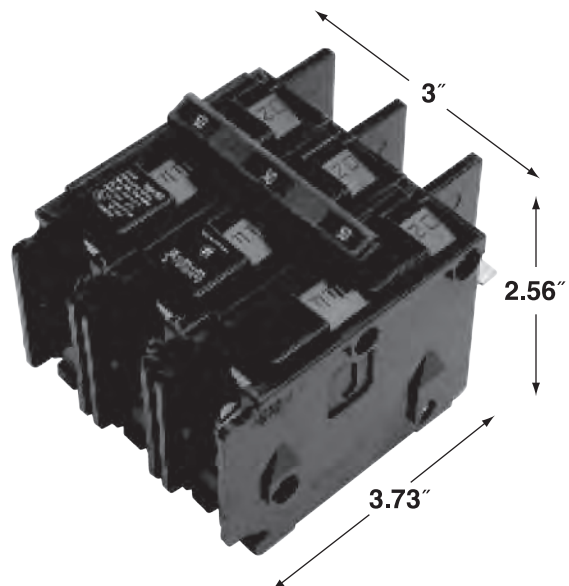
Type BQ Three Pole-Bolt On
