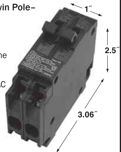
Type QT Twin Pole-Plug In -NC-
