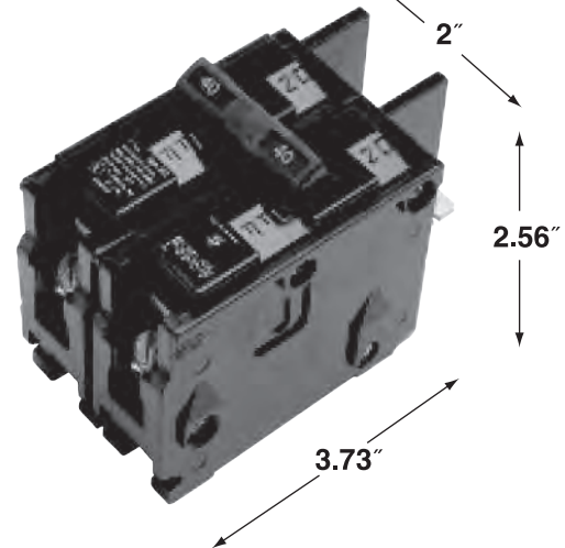
Type BQ Two Pole-Bolt On
