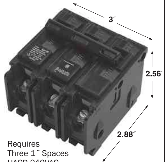
Type QP Three Pole-Plug In
