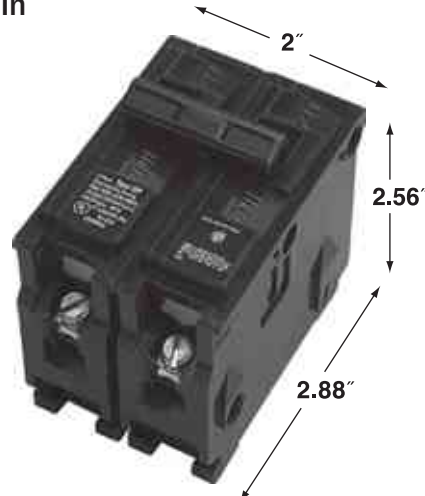
Type QP Two Pole-Plug In
