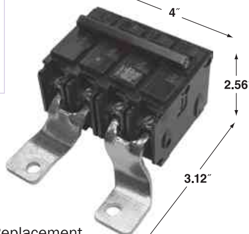
Type MBK Main Breaker
