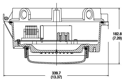
Ceiling Mount
