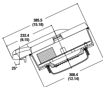
25° Stanchion Mount
