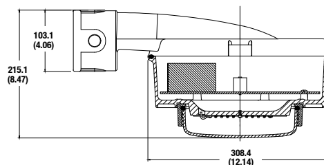
Wall Mount
