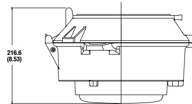
MM-II Adapter-Centric
