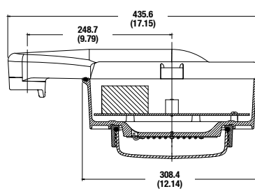
90° Stanchion Mount
